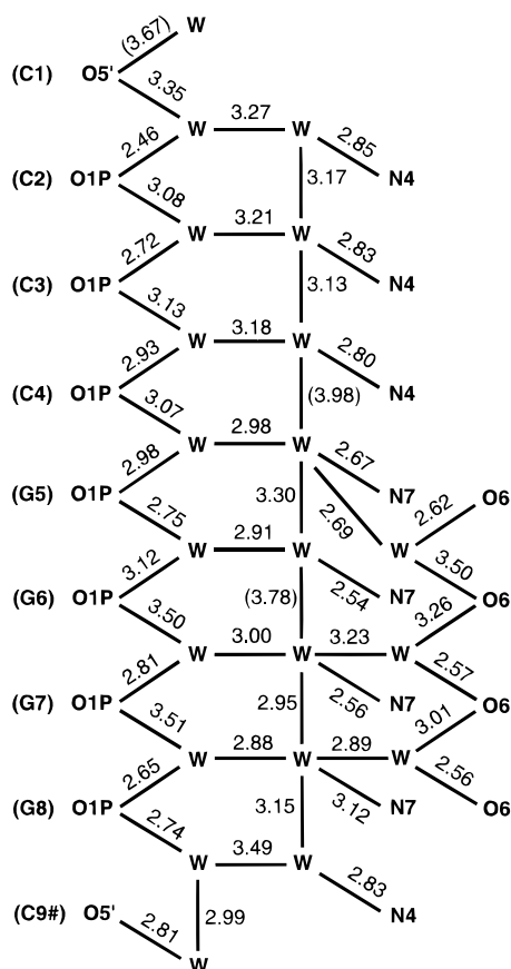
FIGURE 3: Schematic diagram of the longitudinal water structure in the major groove for strand 1 (residues C1 to G8; strand 2 very similar). Distances are in Ångströms and are placed in parentheses where longer than 3.5 Å.
