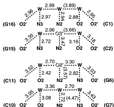
FIGURE 5: Schematic diagram of the second transversal hydration pattern in portions of the duplex, bridging 2'-hydroxyl groups of paired nucleotides approximately within the base-pair plane across the minor groove. Distances are in Ångströms and are placed in parentheses where longer than 3.5 Å. RNA atoms from neighboring duplexes replacing water molecules in the hydration motif are drawn with outline font.
