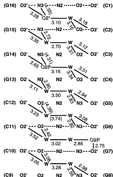
FIGURE 4: Schematic diagram of the transversal water structure in the minor groove, bridging 2'-hydroxyl groups of adjacent residues from opposite strands across the narrowest dimension of the groove. Distances are in Ångströms and are placed in parentheses where longer than 3.5 Å. RNA atoms from neighboring duplexes replacing water molecules in the hydration motif are drawn with outline font. Water bridges across the groove and roughly within the planes of base pairs are included as dashed lines.
