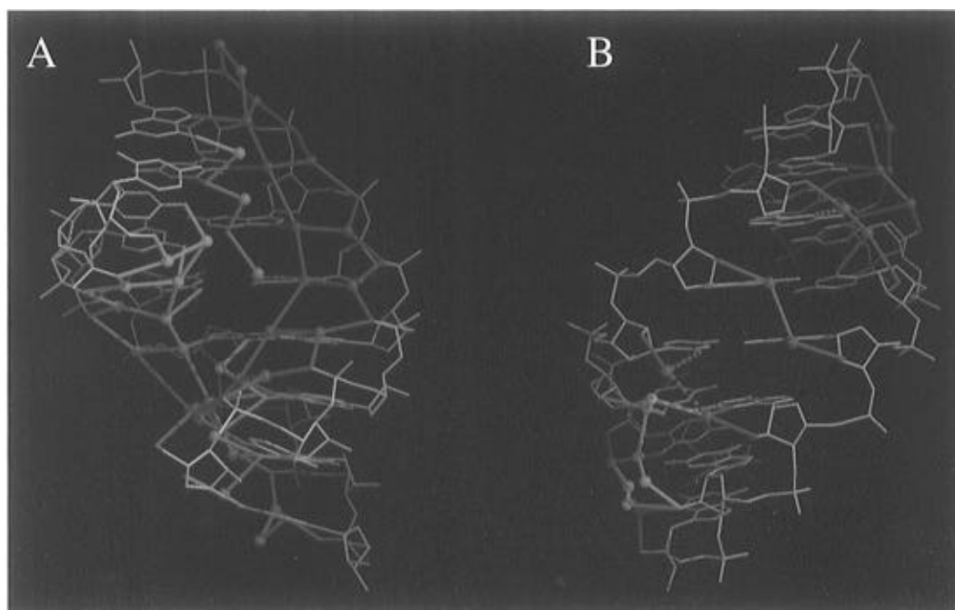
FIGURE 2: Overall views of the hydration patterns in the RNA (A) major and (B) minor grooves (related by a rotation of ca. 180° around the horizontal). RNA atoms are white, and bright portions are closer to the reader. In the major groove, water pentagons along strand 1 are red, along strand 2 they are green, and water bridges between O6 atoms of guanines are yellow and cyan in the top and bottom halves of the duplex, respectively. In the minor groove, water bridges between 2'-hydroxyl groups from opposite strands within base-pair steps are red (dotted for distances >3.5 Å). Bridges between 2'-hydroxyl groups within base-pair planes and sharing a water molecule with the former bridges are cyan. Two water molecules and a phosphate oxygen from an adjacent duplex link the hydroxyl groups of residues G7 and C11 and are colored yellow.
