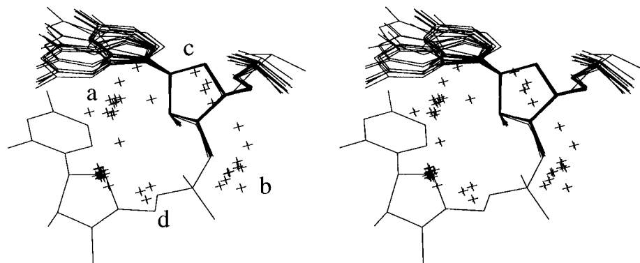
FIGURE 1: Distribution of water molecules (crosses represent oxygen positions) around the ribose 2'-hydroxyl groups within a distance range of 3.5 Å for 16 nucleotides (bold) in [r(C_4G_4)]_2 . The four clusters are labeled a, b, c, and d. The superposed nucleotides (top residues) all adopt C3'-endo type puckers, and the 5'-adjacent residue was included to provide for a typical environment of the ribose. The locations of 5'-adjacent O4' oxygens were included for comparison, independent of whether the corresponding O2'...O4' contact was shorter than 3.5 Å or not, and are discernible as tightly clustered crosses around the O4'-position of the bottom residue.
